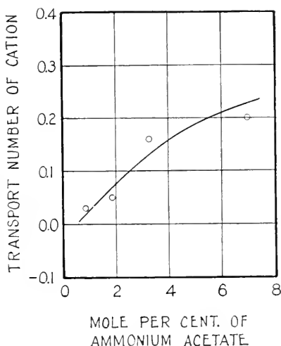
FIG. 3. Apparent transport number of cation in ammonium acetate solutions.
